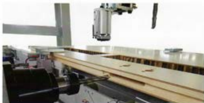
Lavorazione cerniere, serratura e sfinestratura Lock, hinges and window opening operations
